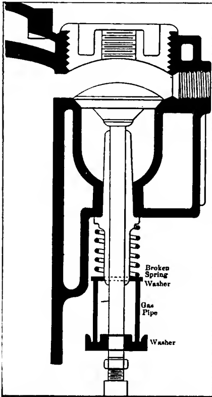
Fig. 1—Method of temporarily repairing a broken valve spring with a piece of gas pipe
